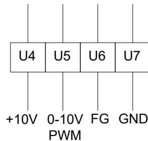
Control Line
