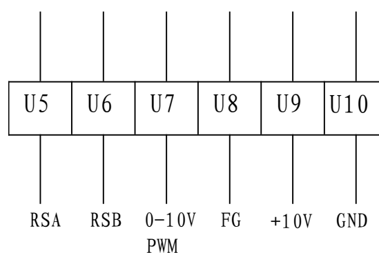
Control Line
