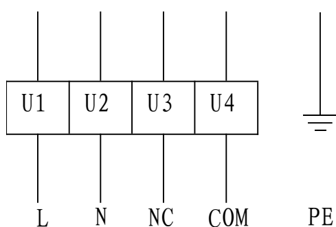
Power Line
