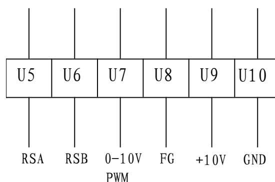
Control Line
