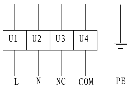
Power Line
